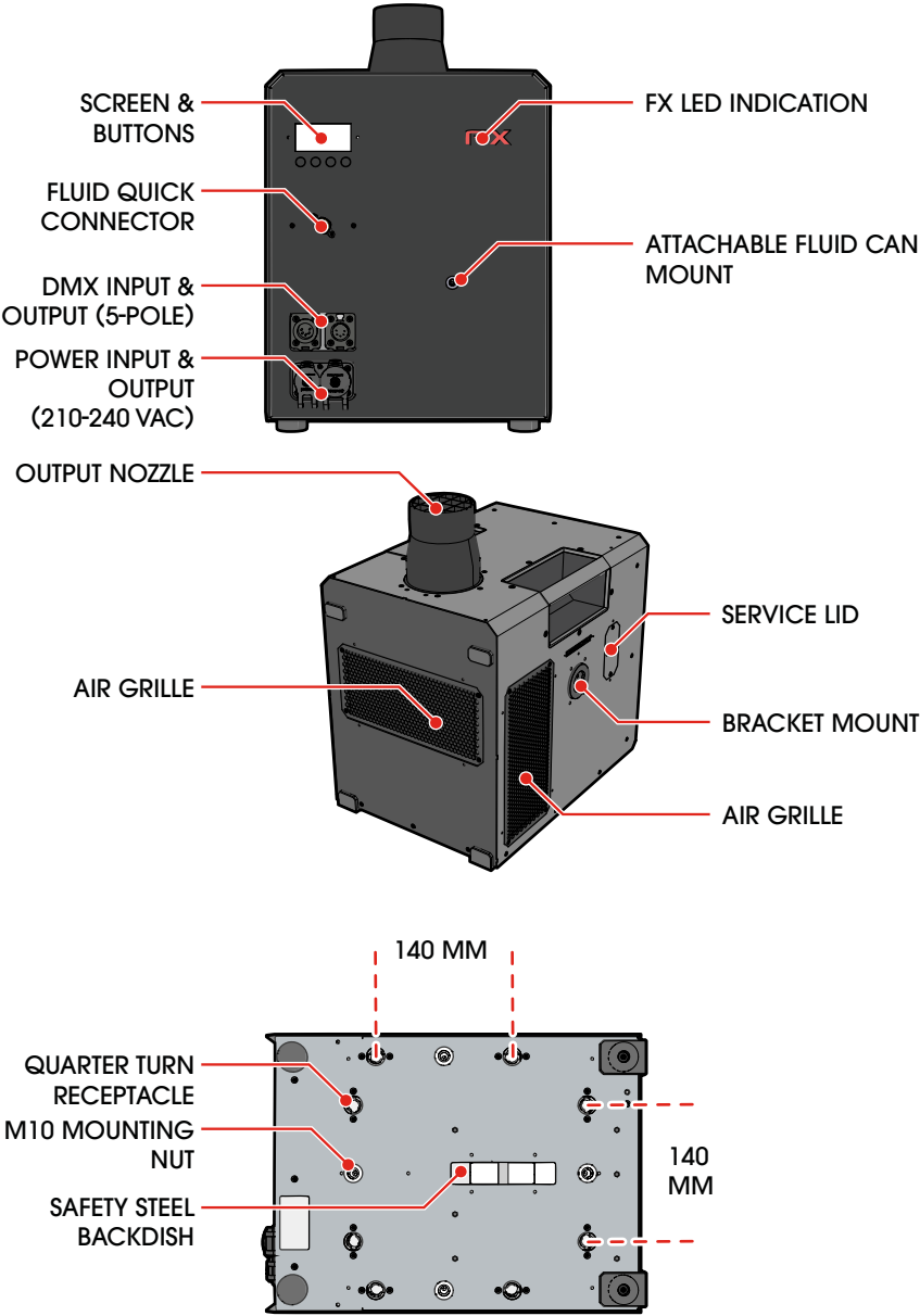
Main parts
